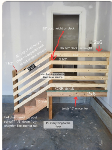
Rail layout - equal spacing, worked top-down
